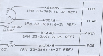
1 - 1 INSTALLATION
