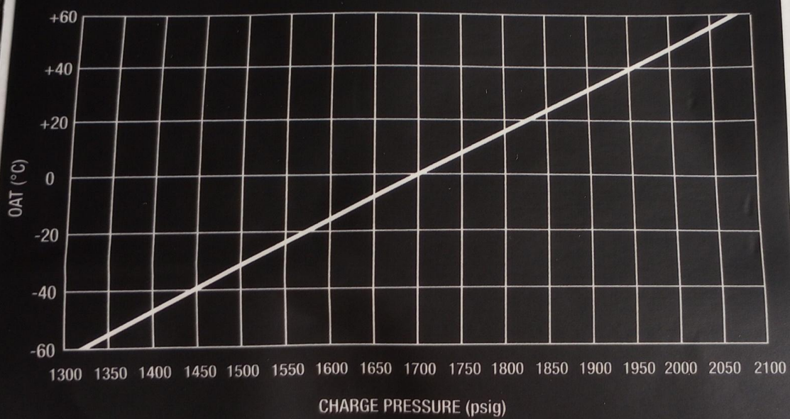
OXYGEN BOTTLE CHARGE PRESSURE V.S. OAT
